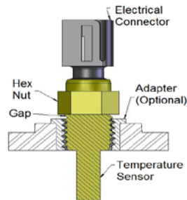
Figure 1: Temperature sensor with adapter bushing.
