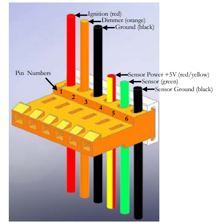
Figure 2: Connector.
