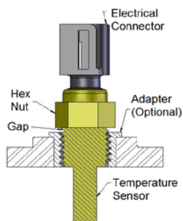
Figure 1: Temperature sensor with adapter bushing.
