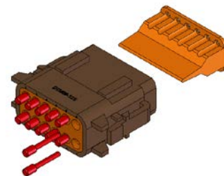
Figure 2: Remove plugs and wedge-lock as shown. Wedge-lock is replaced once wires are positioned properly.
