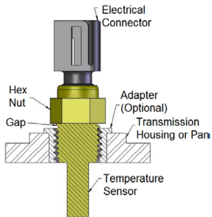
Figure 3: Temperature sensor with adapter bushing.
