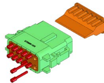
Figure 2: Remove plugs and wedge-lock as shown. Wedge-lock is replaced once wires are positioned properly.
